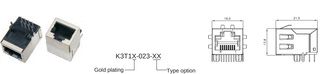
Side Entry Transformer Jack STP (Stamp)
