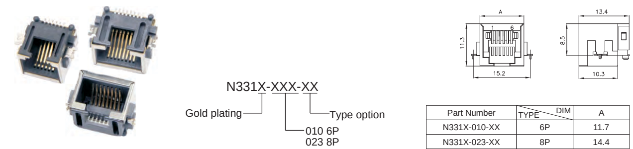
Side Entry 6P SMT Jack UTP (Stamp)
