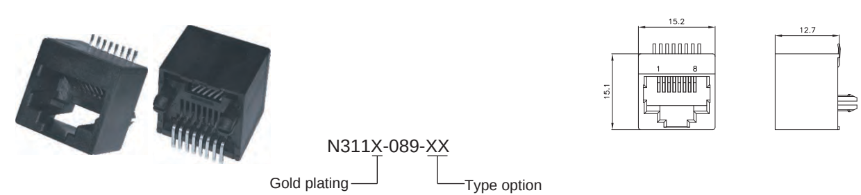
Top Entry 8P SMT Jack UTP (Stamp)
