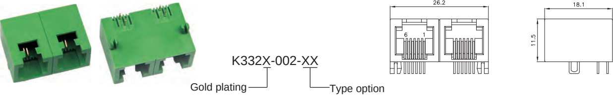
Side Entry 6P PCB Jack UTP (Round)
