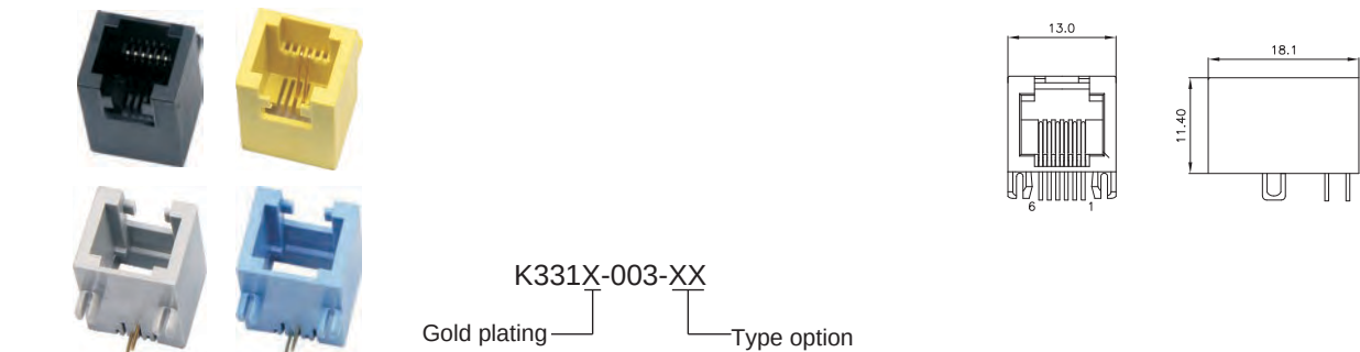
Side Entry 6P PCB Jack UTP (Round)
