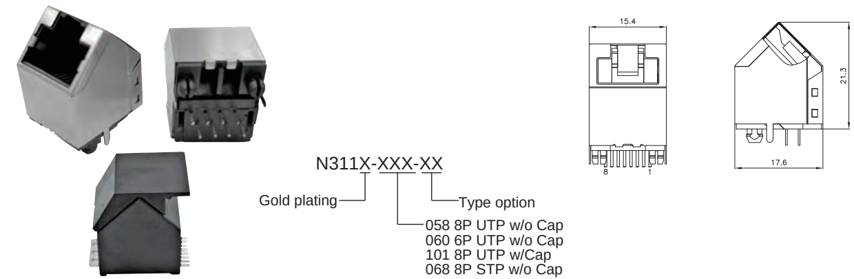
45° 6P、8P PCB Jack (Stamp)
