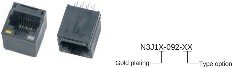
Top Entry LED 8P Jack UTP (Stamp)
