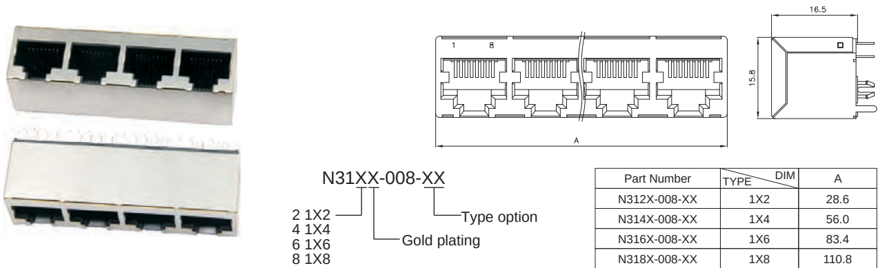
Top Entry 1XN 8P PCB Jack STP (Stamp)
