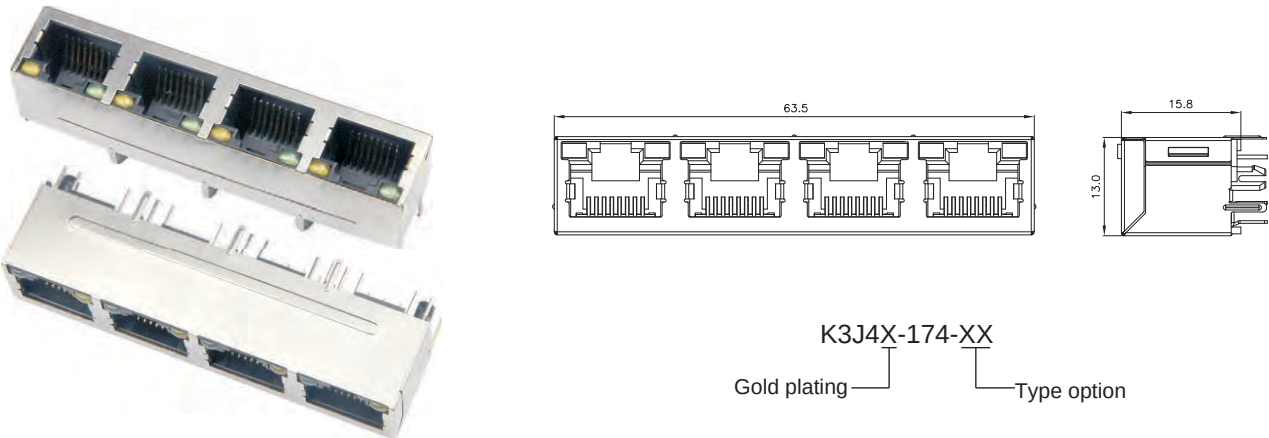
Top Entry 1X4 LED 8P Jack STP (Stamp)
