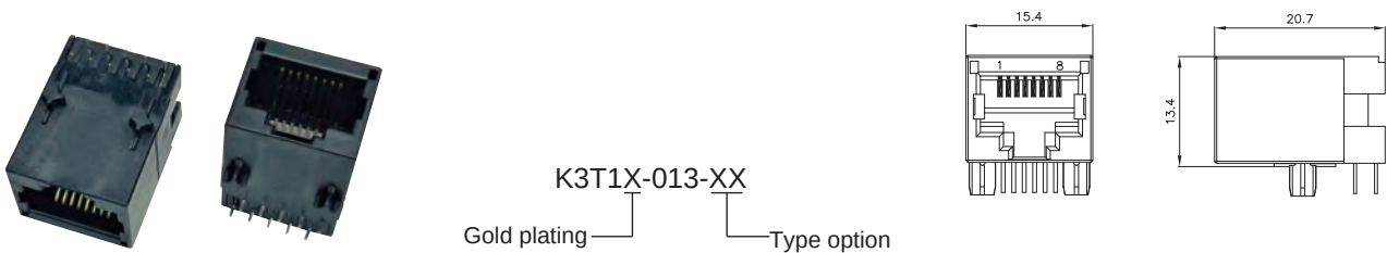
Side Entry LED Transformer Jack STP (Stamp)
