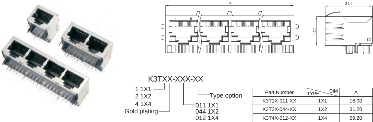
Side Entry LED Transformer Jack UTP (Stamp)
