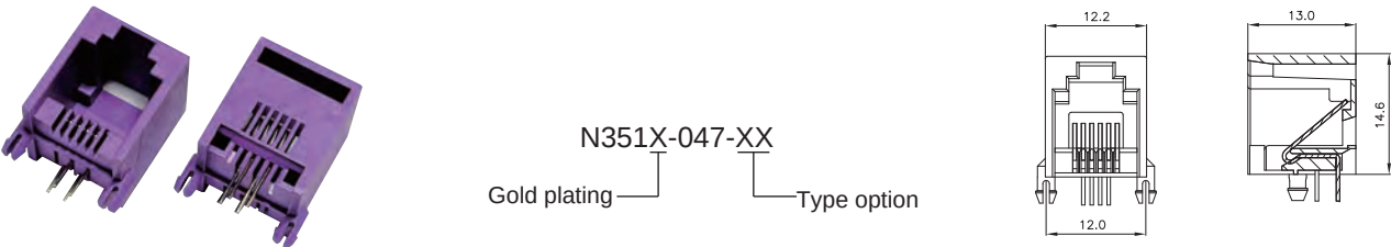
Side Entry 1X2 Mini L/P 6P PCB Jack (Round)
