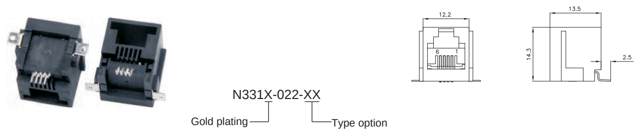
Side Entry 6P SMT Jack UTP (Stamp)
