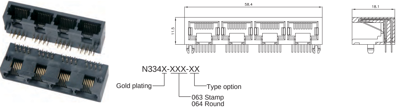
Side Entry 8P RJ31 PCB Jack UTP 1&4/ 5&8 Shorting (Round)
