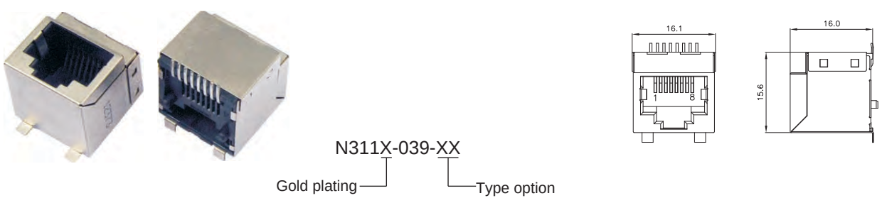
Top Entry 8P SMT Jack STP (Stamp)
