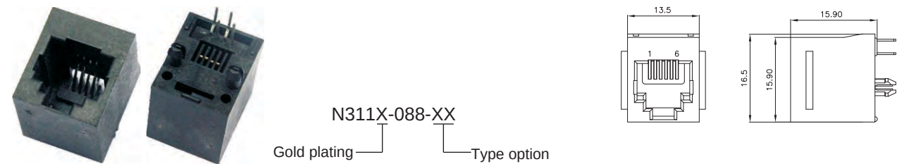
Top Entry 6P PCB Jack UTP (Stamp)
