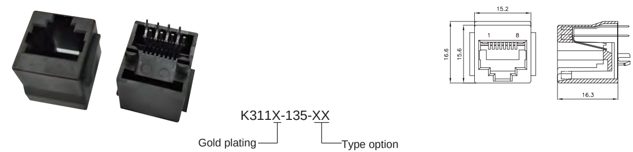
Top Entry 8P SMT Jack UTP (Stamp)
