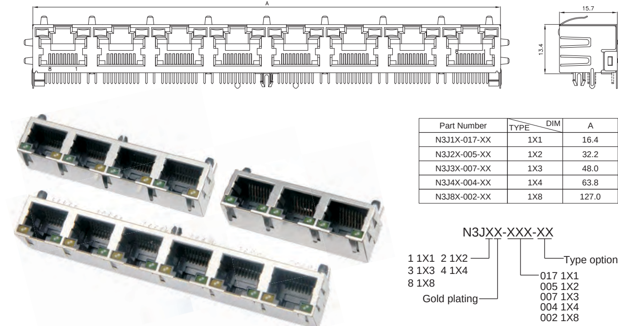
Side Entry LED 1XN 8P Jack STP (Stamp)
