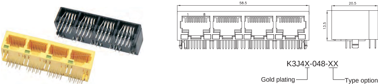
Side Entry LED 1XN 8P Jack STP (Stamp)
