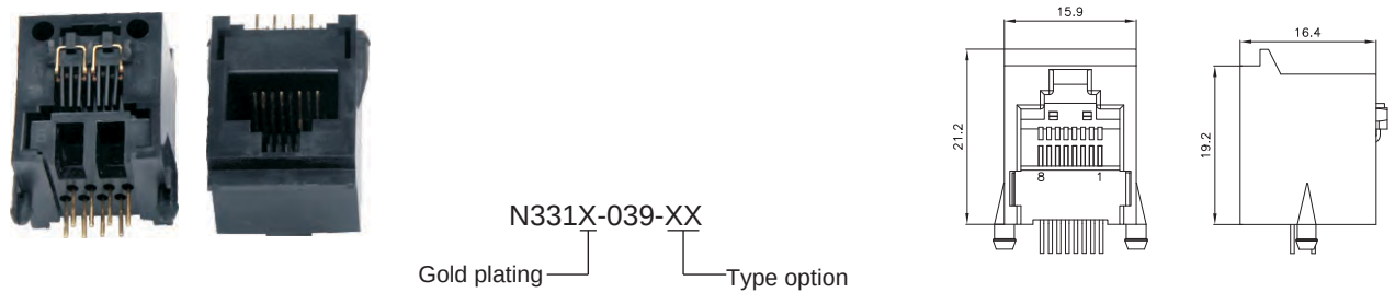
Side Entry 6P、 8P SMT Jack Sunk Type STP (Stamp)
