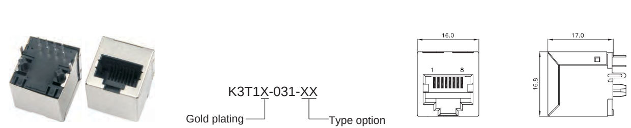
Top Entry Transformer Jack STP (Stamp)
