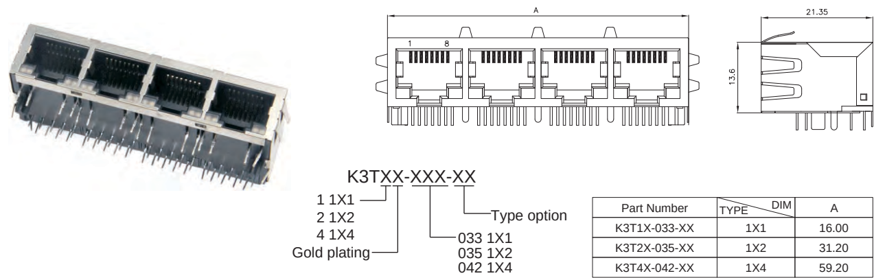
Side Entry LED Transformer Jack STP (Stamp)
