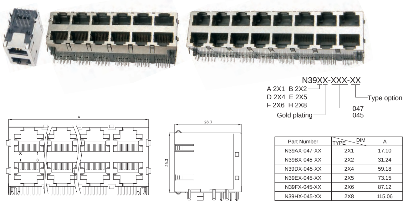
Side Entry 2XN 8P Stacked PCB Jack (Stamp)
