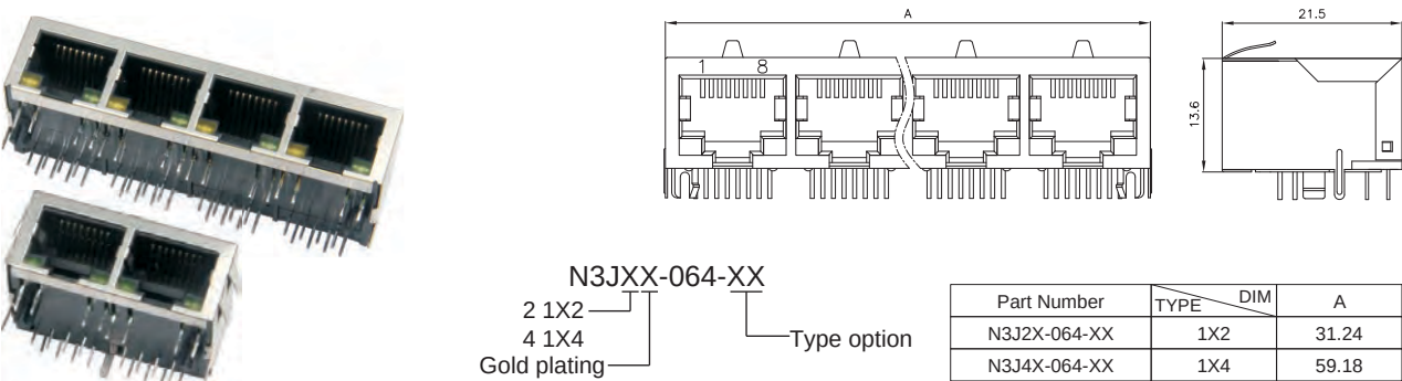
Side Entry LED 1X4 8P Jack UTP (Stamp)
