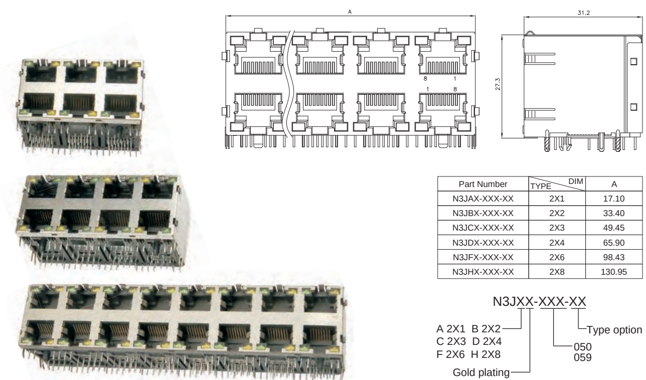
Side Entry LED 2XN 8P Stacked Jack STP (Stamp)
