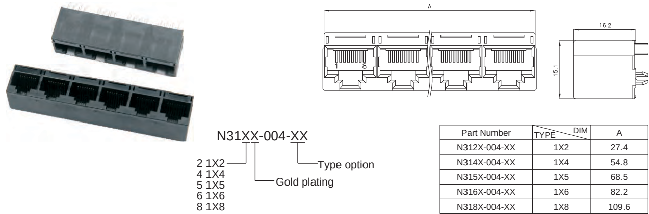
Top Entry 1XN 8P PCB Jack UTP (Stamp)
