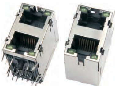
Side Entry LED 2X1 8P Stacked Jack STP
