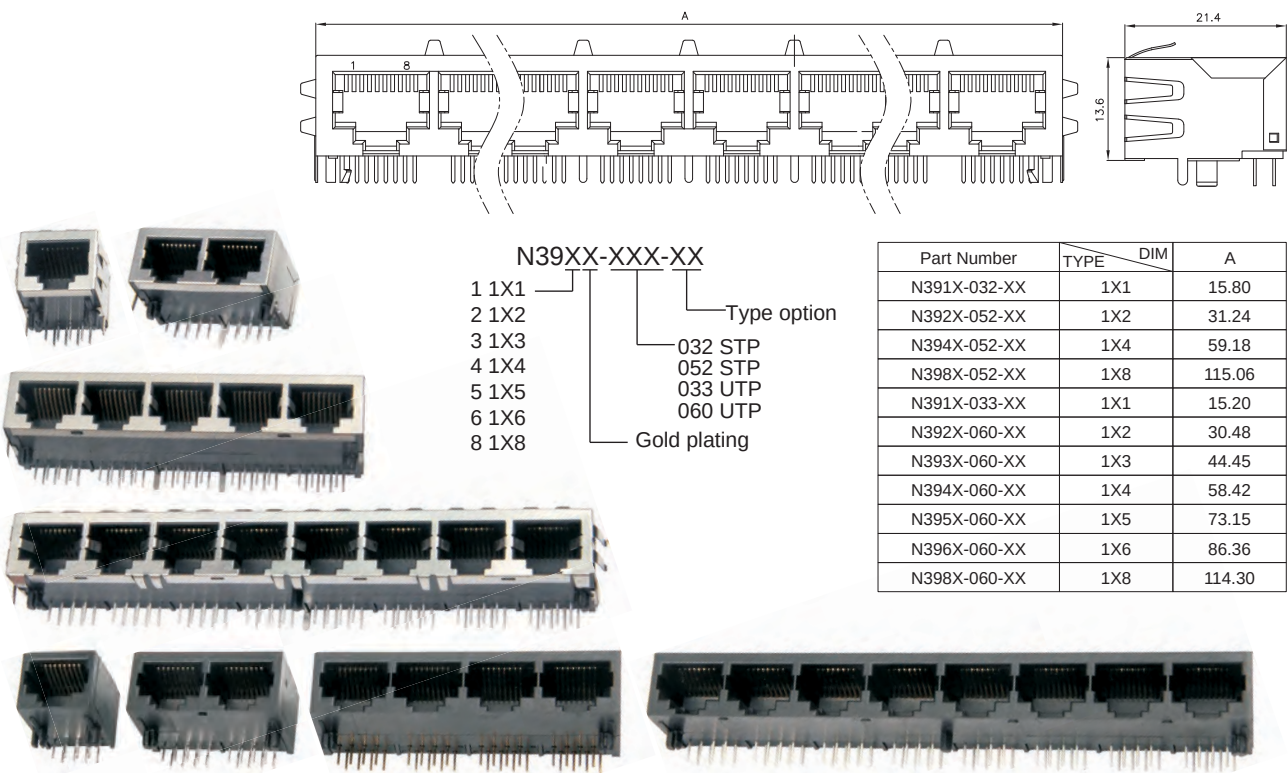
Side Entry 1XN 8P PCB Jack (Stamp)
