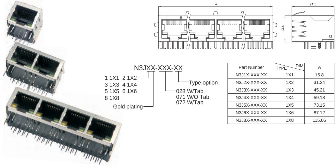
Side Entry LED 1XN 8P Jack STP (Stamp)
