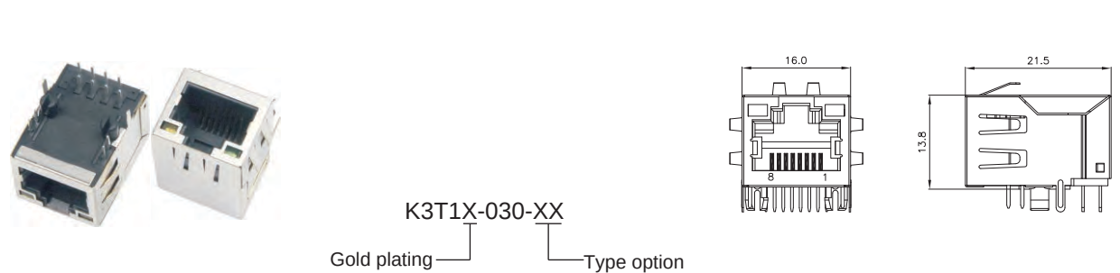
Side Entry LED Transformer Jack STP (Stamp)
