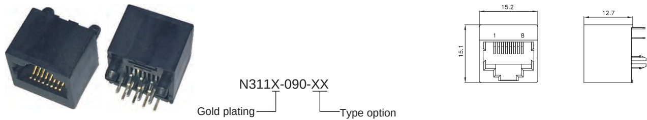
Top Entry 8P PCB Jack DIP UTP (Stamp)
